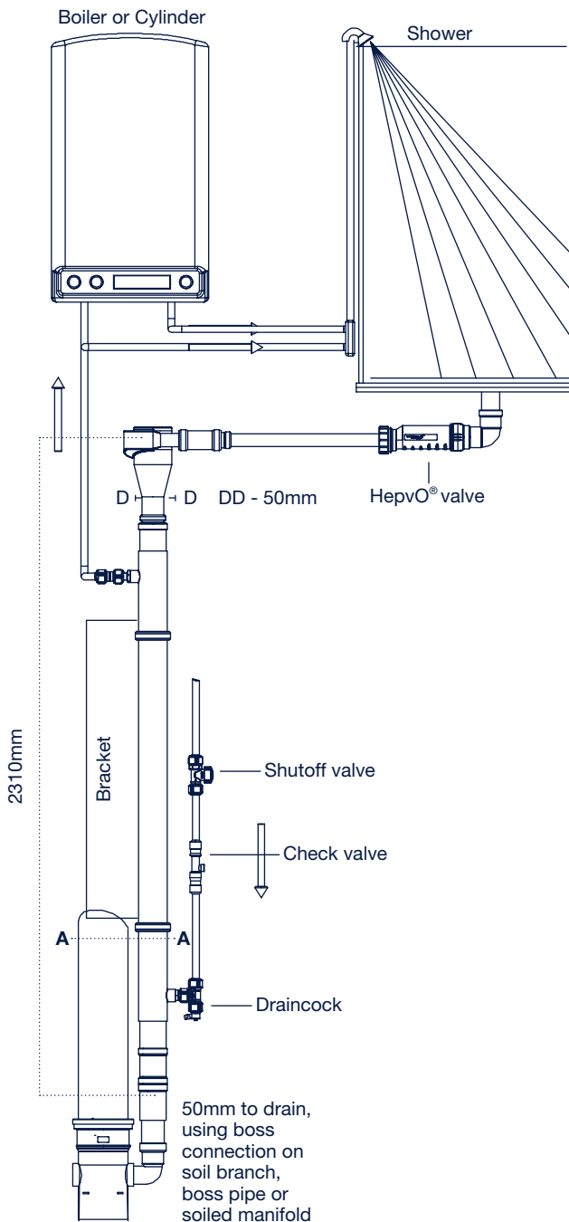
Fig.1 Side View
